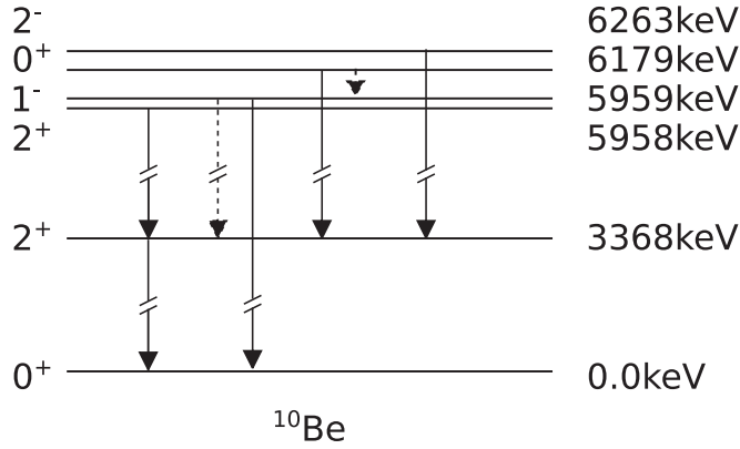
Figure 1. Level scheme of the bound states in ^{10}\text{Be} . The excitation energy, spin and parity are given. The gamma decay lines with a branching ratio larger than 10% are shown as well. In the levels with more than one decay, the decay with the largest branching ratio is marked with a solid line.
