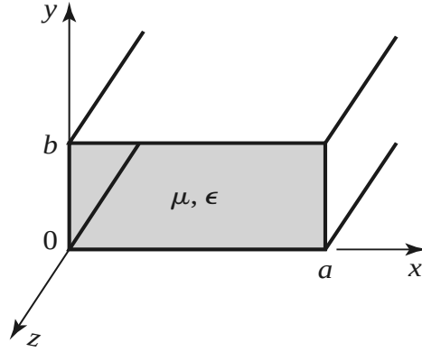
Figure 1.3: The geometry of a rectangular waveguide.
