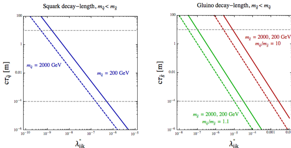
Figure 5. The decay lengths of a squark (left) and a gluino (right).
