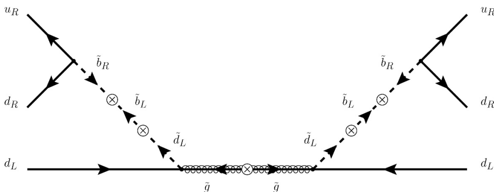
Figure 7. The Barbieri and Masiero diagram contributing to BM_1 .
