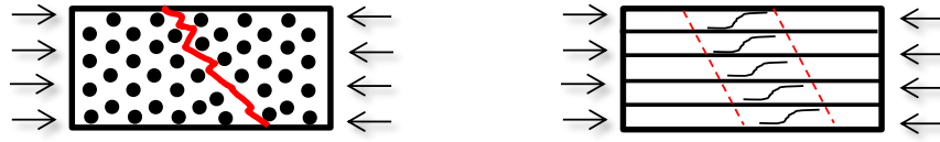
Figure 4: Compressive failure modes of a UD ply. Left: Transverse compression. Right: Kinking failure in longitudinal compression. Courtesy of [22].
