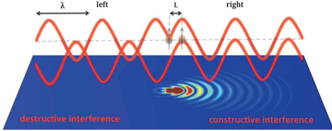
Figure 2.2: Schematic illustration of the net radiation pattern from a pair of detuned dipole emitters when conditions for total constructive/destructive interference are fulfilled. The upper rays illustrate the radiation from an individual dipole emitter while the lower plane shows the resulting interference pattern in opposite directions along the dimer axis.
