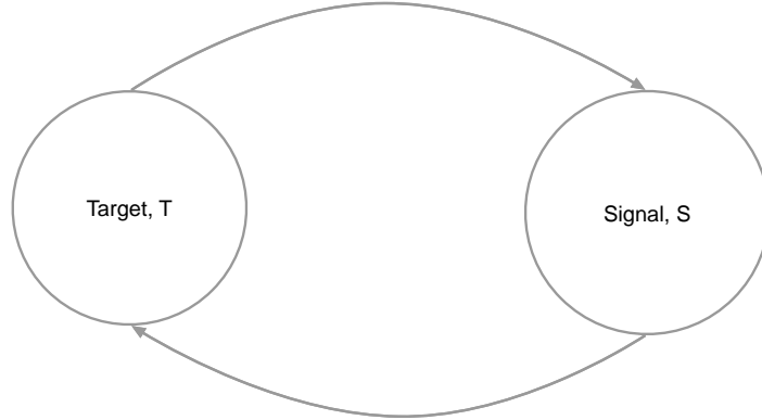
Figure 4.1: Principle of retrieving a signal or a target for remote sensing. The target T represent an atmospheric state and the signal S represent a radiometric measurement.
