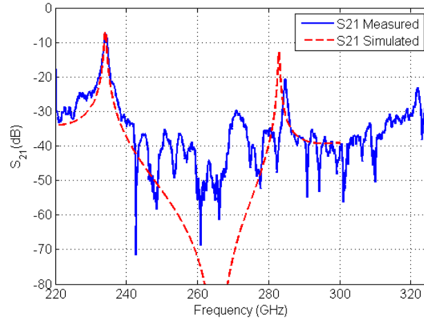
Figure 6: Measurement and simulation of the previous Si ridge gap resonator, [8].
