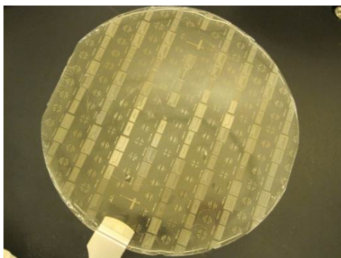
Figure 9: A complete SU8 wafer.
