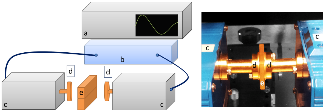
Figure 5: Measurement setup with a photo of the resonator being measured. a) The network analyzer (Agilent N5250C), b) The millimeter-wave controller (Agilent N5260A), c) OML extender, d) WR03 flange, e) Support package for the resonator (Fig. 4).
