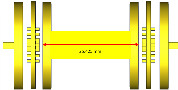
Figure 13: Measurement setup for comparing the straight rectangular waveguide with pin flanges between the waveguide and the measurement flanges on both sides. (Spacers not shown in the figure)
