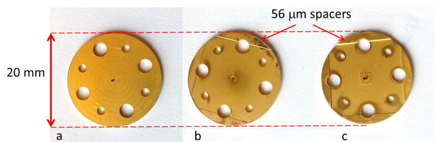
Figure 11: a) The 1 mm waveguide disc, b) the milled choke flange, c) the milled pin-flange.
