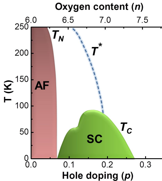
Figure 2.2: Phase diagram of YBa 2 Cu 3 O 7-δ , as a function of both hole doping p per planar copper atom and oxygen content n per unit cell. T_N , T^* and T_C are respectively the Néel, the pseudogap and the critical temperature. (Adapted from [53])
