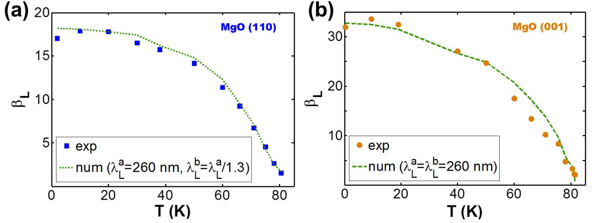
Figure 6.3: Comparison between the experimental (dots) and the theoretical (lines) values of the screening inductance factor \beta_L as a function of the temperature for nanoSQUIDS patterned on (a) a MgO (110) substrate, considering for the fit a \lambda_0^a value of 260 nm and the in-plane anisotropy of the London penetration depth; (b) a MgO (001) substrate, considering for the fit a \lambda_0^a value of 260 nm and assuming the in-plane isotropy of the London penetration depth.
