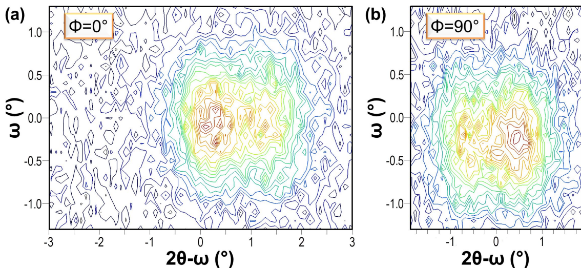
Figure 3.11: XRD 2\theta - \omega maps around the (308)/(038) reflections of YBCO (a) fixing \phi = 0^\circ (the center of the scan in 2\theta is 105.3^\circ ); (b) \phi = 90^\circ (the center of the scan in 2\theta is 106.1^\circ ). In both the cases the tilt angle \chi has been chosen so to get different intensities from the two peaks, highlighting the two distinct reflections, which occur at 2\theta = 105.4^\circ and 2\theta = 106.6^\circ . From the position of these two peaks we can extract the following in-plane parameters: a = 3.82 \text{ \AA} , b = 3.88 \text{ \AA} , which are rather close to the relaxed values.
