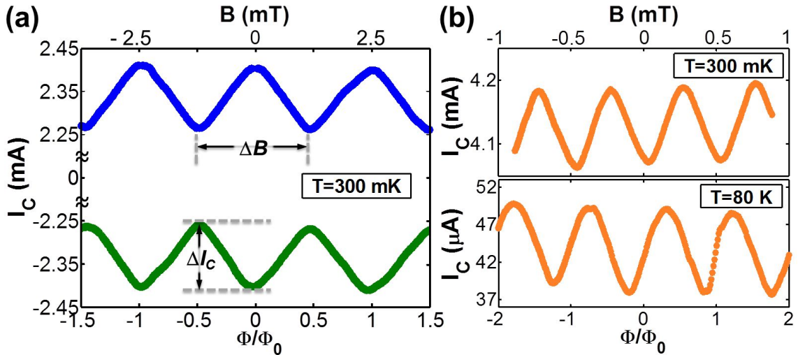
Figure 6.2: Critical current as a function of the applied magnetic field measured (a) at 300 mK, on a device patterned on MgO(110) with a loop area of 130 \times 150 nm ^2 ; (b) at T=300 mK ( upper panel ) and close to T_C ( lower panel ), on a device patterned on MgO(001) with a loop area of 130 \times 1000 nm ^2 .
