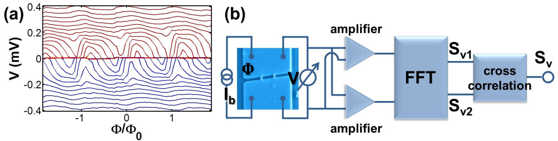
Figure 6.6: (a) Voltage modulations of the nanoSQUID mentioned in Fig. 6.5. V(\Phi) are shown for I = [-2.5, 2.5] mA (in 26 \mu\text{A} steps), among which a voltage modulation of 0.2 mV (peak-to-peak) is present, corresponding to a transfer function V_\Phi = 1.5 \text{ mV}/\Phi_0 . (b) Basic scheme of the setup used for our noise measurements. The nanoSQUID is biased in current and in magnetic flux. The voltage signal from the device is fed to two independent input amplifiers operating in parallel, followed by a two-channels FFT dynamic system analyzer operated in cross correlation mode. The voltage noise from the nanoSQUID is coherent and correlated in both channels and averages to a finite value. The frequency components of the noises of the two input amplifiers are uncorrelated and they can be reduced by a proper averaging.
