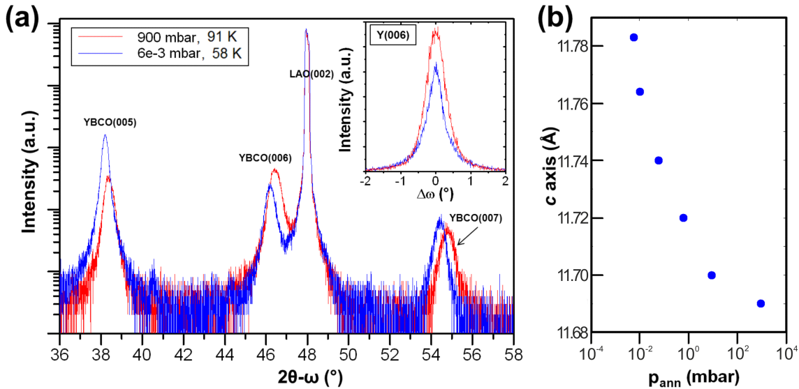
Figure 3.13: (a) XRD 2\theta - \omega scans of an optimally doped YBCO film and of an underdoped film, with the lowest critical temperature ( T_C \approx 58 K). All the (00n) peaks of the underdoped film are shifted toward the left. In the inset, the rocking curves of the (006) peak of these two films are shown, both characterized by a FWHM narrower than 1^\circ . (b) The c -axis lattice parameters of YBCO, extracted from the position of the (00n) Bragg peaks in the XRD 2\theta - \omega scans, are shown as a function of the in-situ post-annealing pressure.
