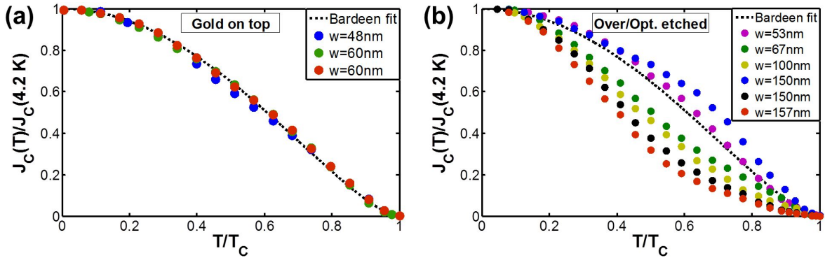
Figure 5.7: Normalized critical current density J_C(T)/J_C(4.2 K) measured in the whole range of temperature for nanowires capped with gold (panel (a)) and for those whose Au capping layer has been removed (panel (b)).
