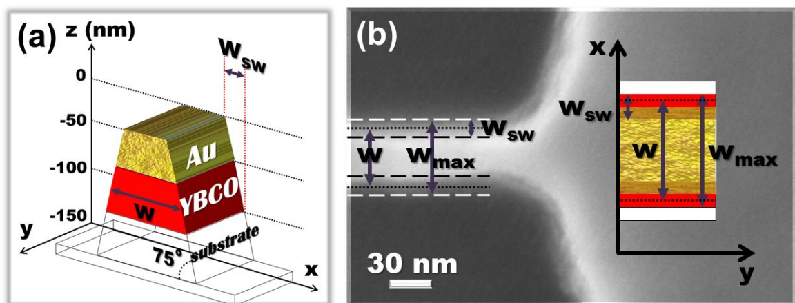
Figure 4.3: (a) Schematics of a typical AFM line scan along the cross section of a nanowire. (b) a SEM picture of a nanowire is combined to the schematics of the top view of the AFM cross section, showing the wire from the SEM perspective. The w can be calculated as w = w_{max} - w_{sw} .
