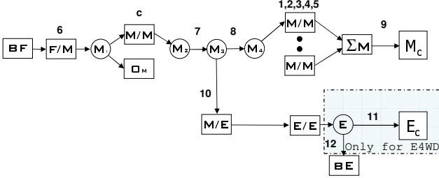
Figure 7: Abstraction model of a parallel PS with ICE, ISG, clutch, and automated manual GB, with Chassis connections: Mechanical-'Mc' and Electrical-'Ec'.
