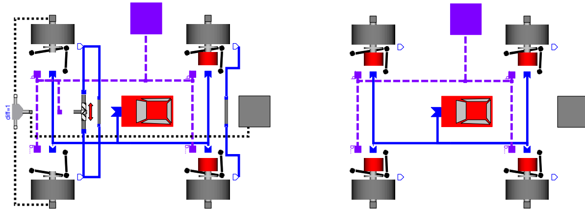
Figure 9: Chassis models corresponding to the first configuration (left) and the second configuration (right).
