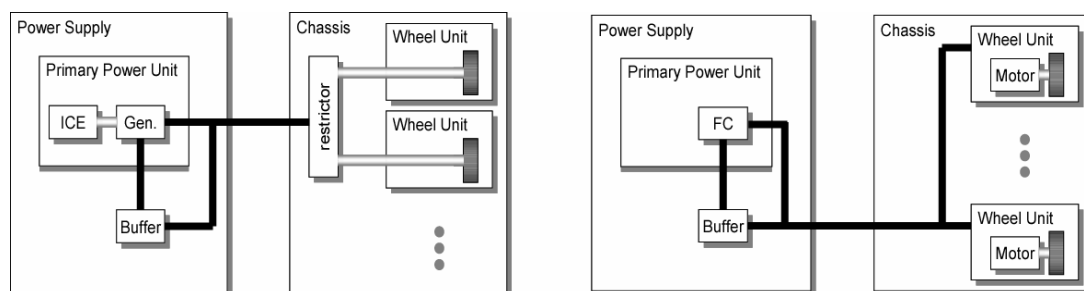
Figure 5: Illustration of power supply for serial with internal combustion engine (left) and serial with fuel cell (right) HEV configuration. ICE=Internal Combustion Engine, Gen=Generator, FC=Fuel Cell, Black line=electrical power, and Grey line=mechanical power.
