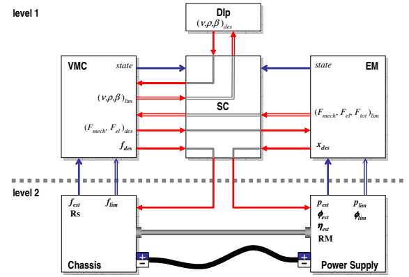
Figure 1: Part of the suggested architecture with focus on the interaction between VMC/Chassis and EM/Power Supply. Double lines indicate limits and single lines are control signals.
