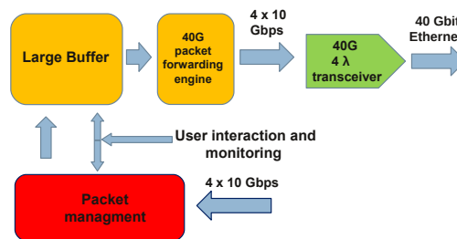
Figure 3: Block diagrams of the FILA40G unit. The data comes into the “packet management” subunit as 4 × 10 Gbps data streams. This subunit will handle additional data processing. From there via the “large buffer” the data flows through the “40G packet forwarding engine” to a 40GE transceiver and on to Ethernet.
