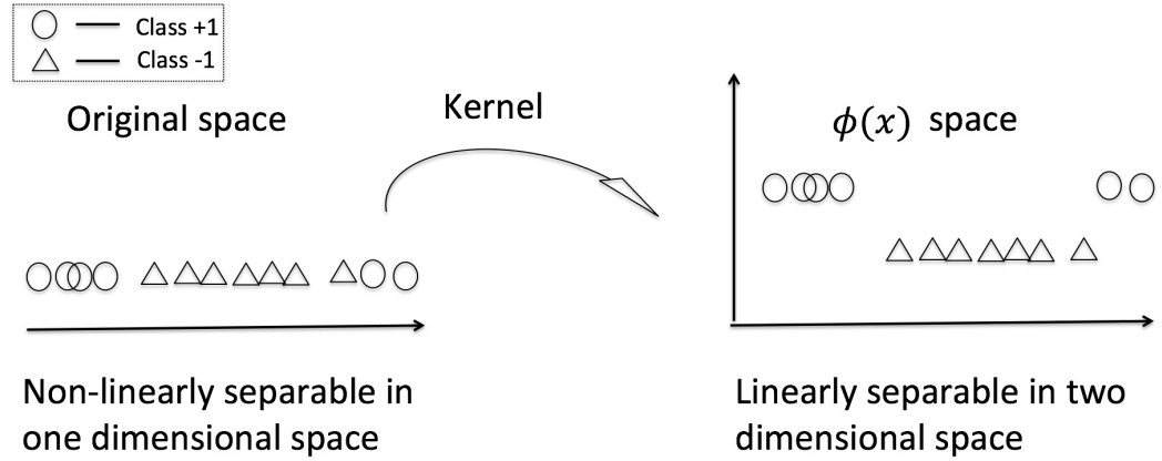
Figure 2.2: Kernel tricks map the data set to a higher dimensional vector space equipped with inner product K without adding any computational complexity.
