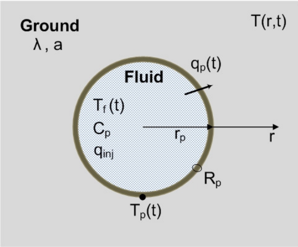
Figure 1.2 The simpler step-response problem for a pipe in the ground.
