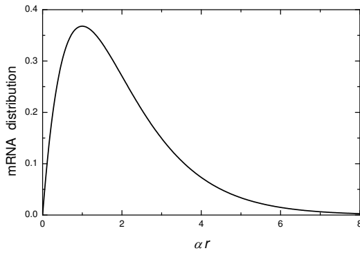
Figure 1. Radial distribution of mRNA according to Eq. (19).
