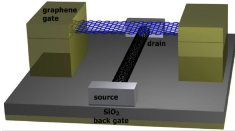
Figure 3.2: A Carbon NanoTube Field Effect Transistor (CNTFET) can be realised by adding to the prototypal NEMS structure a semiconducting nanotube. The graphene sheet is then used as a top gate. The flexibility of the top gate can be shown to enhance the switching of the transistor.
