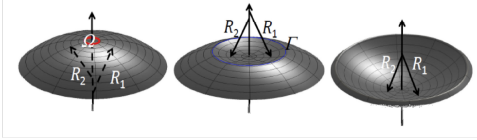
Figure 5.4: A schematic view of the process of snap through. Left: For small pressures a local deformation is formed in the region denoted \Omega . Middle: When the critical pressure is reached, it becomes energetically favourable to form a concave region where the elastic energy is confined to a narrow region \Gamma . Right: This concave region is elastically unstable. As a result, the deformation propagates outward, and the sheet snaps through.
