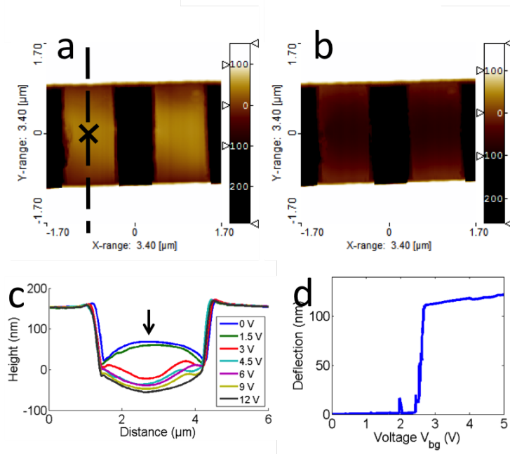
Figure 5.2: A doubly clamped structure showing a snap through instability. a) and b) are AFM images of the sample at 0V and 3V, respectively. In c), AFM sweeps have been made along the dashed line in a) while gradually increasing the voltage. In d) the AFM tip is kept fixed at the spot marked with a cross in a) while gradually increasing the voltage. Here, the snap-through instability manifests itself as the discontinuity in tip position at 2.6V.
