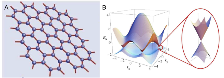
Figure 1.1: A: Schematic image of a graphene sheet, showing the carbon atoms arranged in a hexagonal lattice. B: The electronic spectrum of graphene, showing the linear spectrum close to the Dirac point as an inset. Image adapted from [6].
