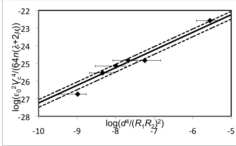
Figure 5.6: Scaling of the snap-through voltage with radius of curvature for fully clamped bilayer drums. The full line is the best least squares fit to the logarithmised values, while the dashed lines represent the uncertainty. The scaling is consistent with theoretical considerations.
