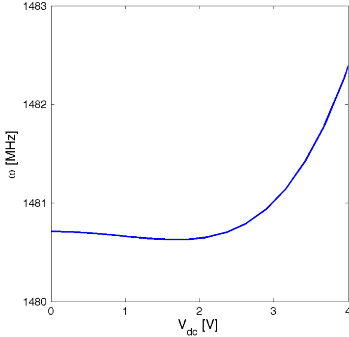
Figure 3.1: The resonance frequency of a suspended graphene sheet with parameters defined in the text, as a function of the bias voltage. The resonance frequency initially decreases slightly as a result of the electronic softening, but then increases again due to the mechanical stiffening of sheets under tension. For even higher frequencies, the electronic softening is expected to again prevail causing the sheet to snap-in to the substrate.
