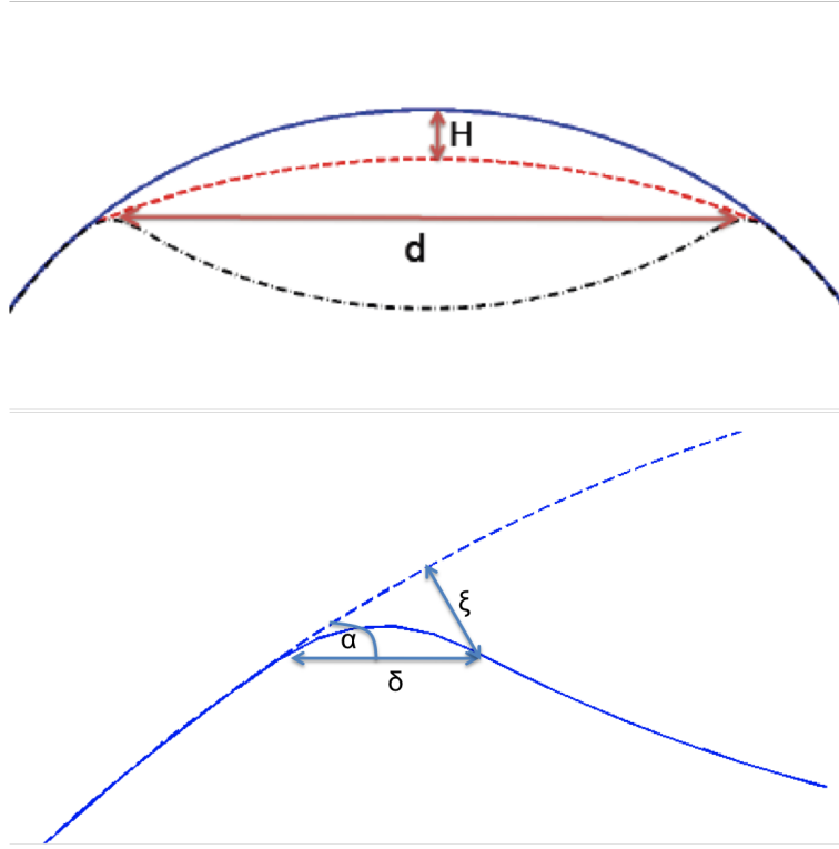
Figure 5.5: Top: Shells under external pressure display two qualitatively different regions of deformation, indicated in the figure by the dashed and dash-dotted line. At low pressures, the shell will locally flatten, decreasing the local curvature. For large pressures, the deformed part of the shell will form a mirror image of its undeformed counterpart. The main contribution to the elastic energy will then be contained in a narrow region close to the edge of the deformed region. Bottom: Close-up of the edge of the deformation for large pressures. The edge region can be parametrised by a width \delta and an angle \alpha .
