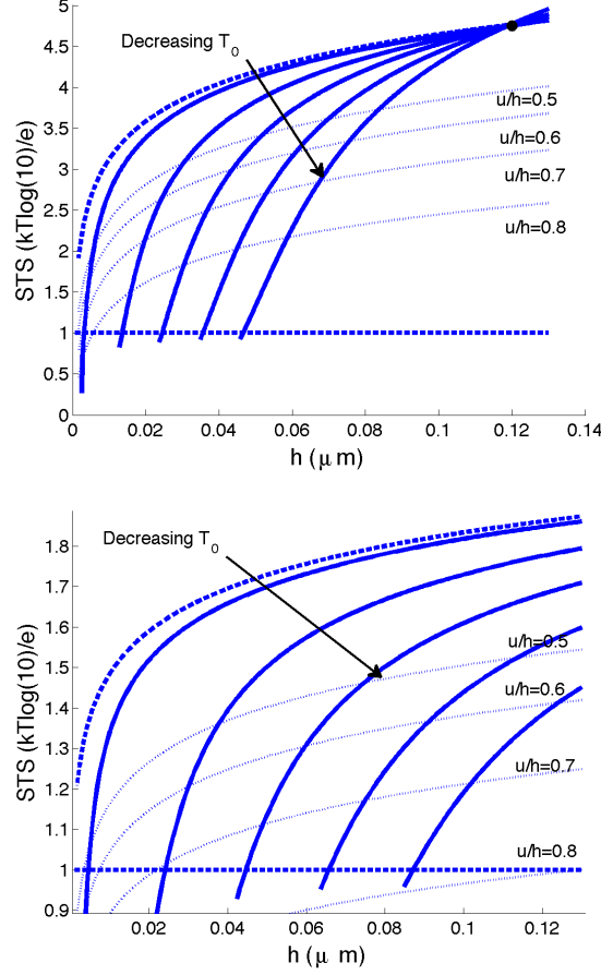
Figure 3.3: The subthreshold slope as a function of the CNT-Graphene gate distance, for various values of u_1 . Upper figure: With parasitic capacitances fitted to the experimental data. In order to avoid snap-in at the thermal limit, the suspension height cannot be larger than 3 nm. Lower figure: Without inclusion of parasitic capacitance. Now, the suspension height can be \sim 10 nm without snapping in at the thermal limit.
