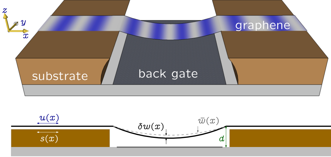
Figure 4.1: Schematic image of a suspended graphene sheet. Note that in the model used in this thesis, the trench enters only as a region of vanishing coupling between the graphene and the underlying substrate
