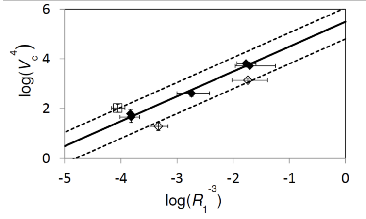
Figure 5.7: Scaling of the snap-through voltage with radius of curvature for doubly clamped beams. The open diamonds are monolayers, full diamonds bilayers and open square trilayer. The scaling is consistent with theoretical considerations.
