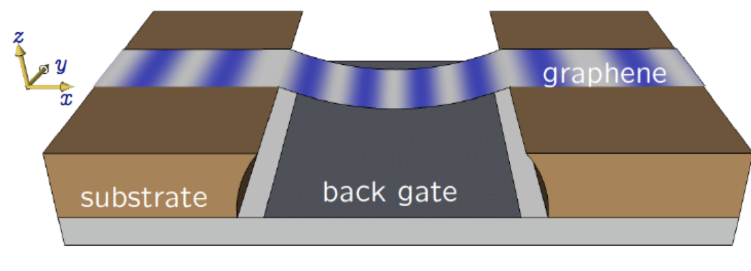
Figure 1.2: A prototypical graphene NEMS structure. A graphene sheet is suspended over a trench in the substrate. Mechanical motion of the graphene is induced by applying a voltage to the gate below it.
